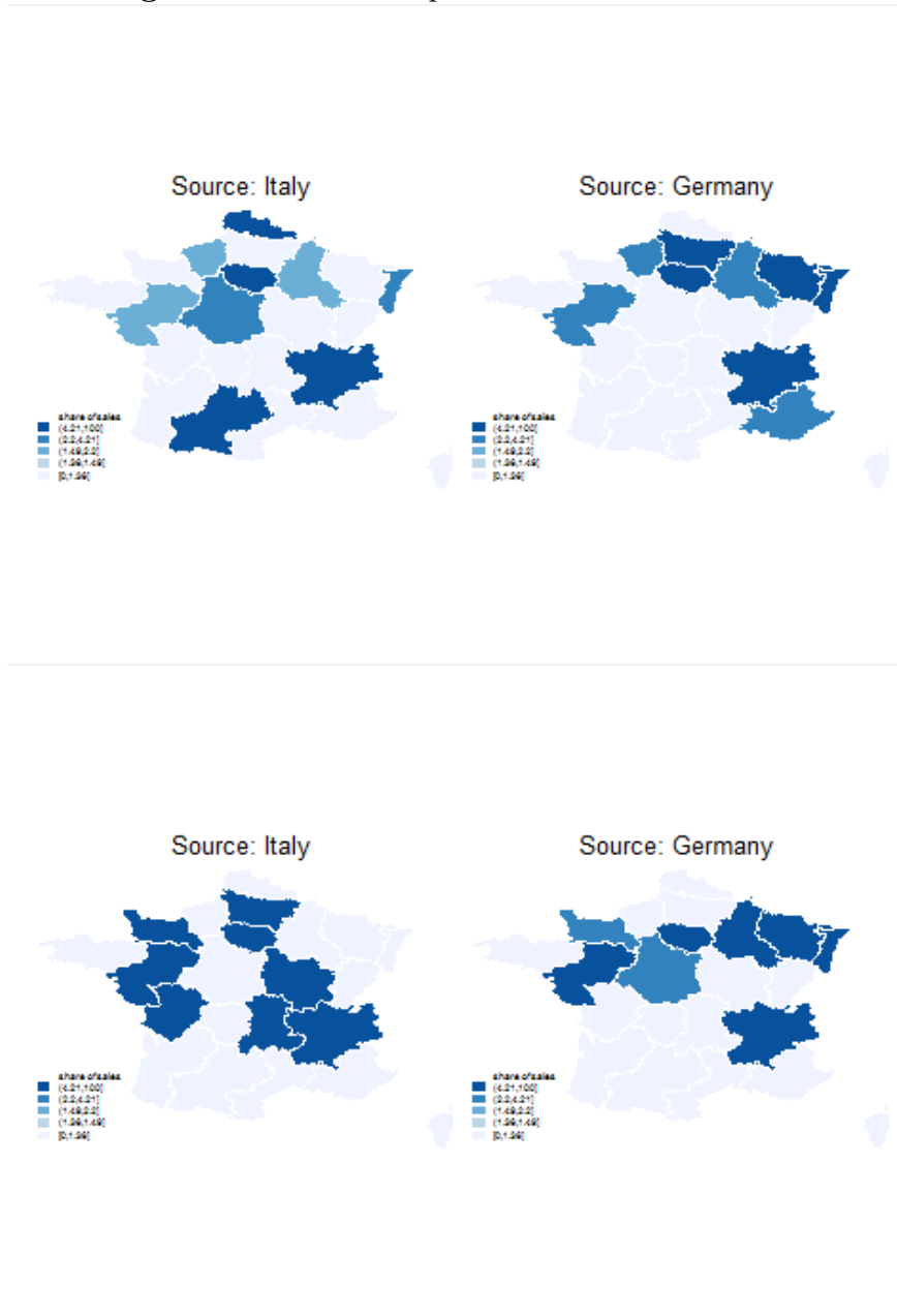
Figure D2. France: Top Panel: Chemicals. Bottom Panel: Transport Equipment
