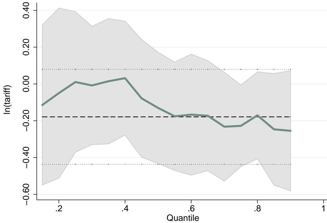
Figure D6. Effect of tariff across U.S. foreign affiliate sales' quantiles
