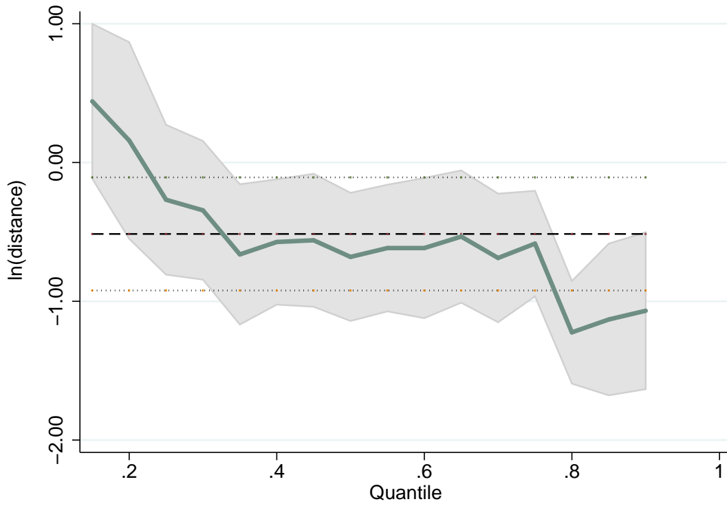
Figure 4. Effect of distance across U.S. affiliate sales' quantiles
